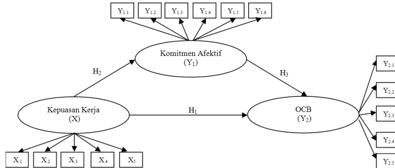
Gambar 1 Model Analisis
