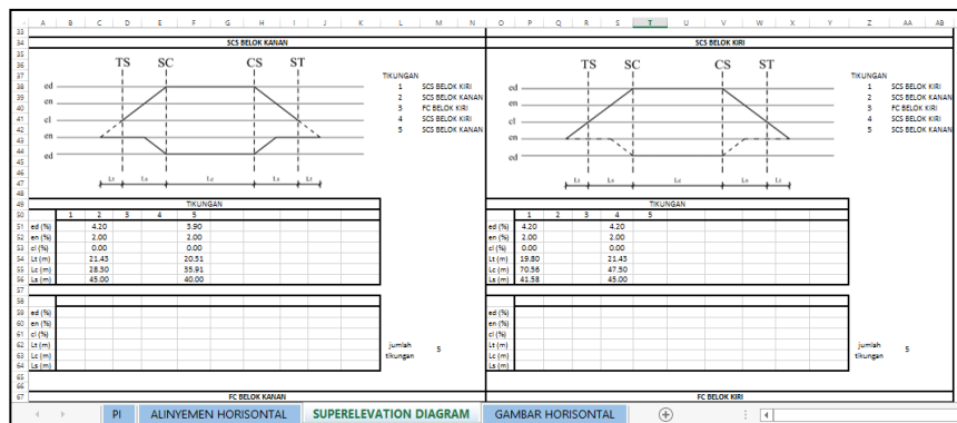
Gambar 4. Hasil Superelevation Diagram
