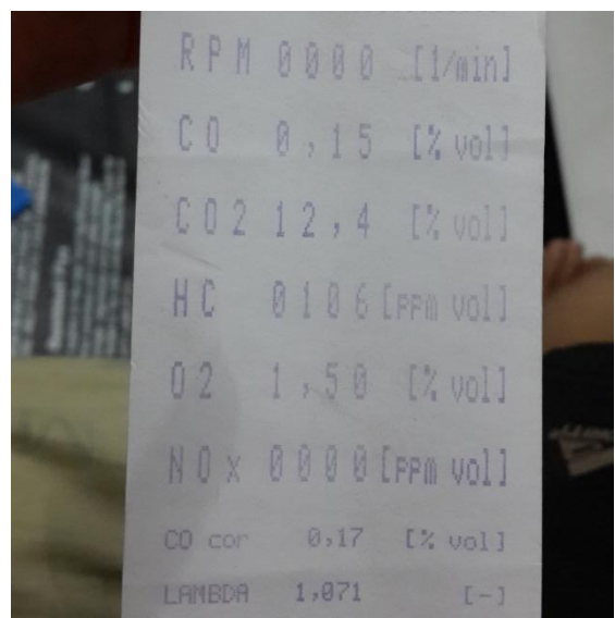
Gambar 9. Hasil Uji Emisi Water Injection
