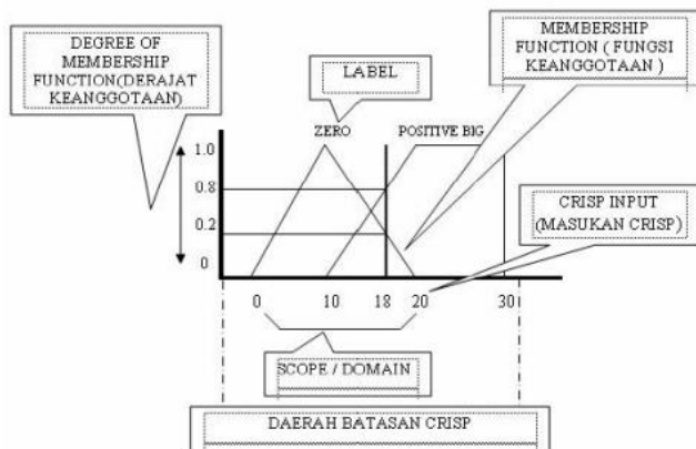
Gambar 1. Fuzzy Logic
