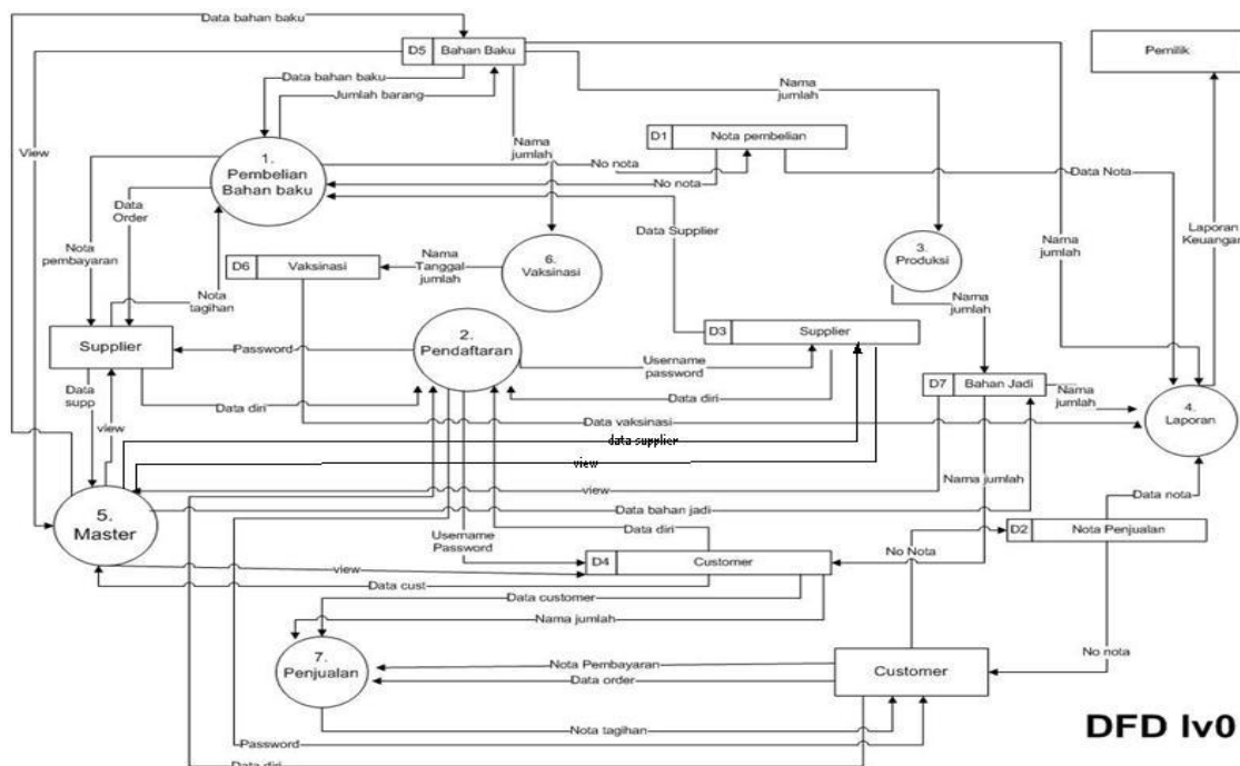
Gambar 1. DFD Level 0
