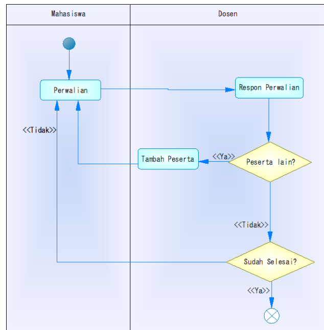
Gambar 1 Activity Diagram
