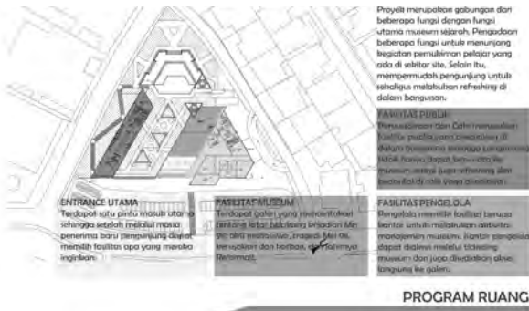
Gambar 2.18 Program Ruang
