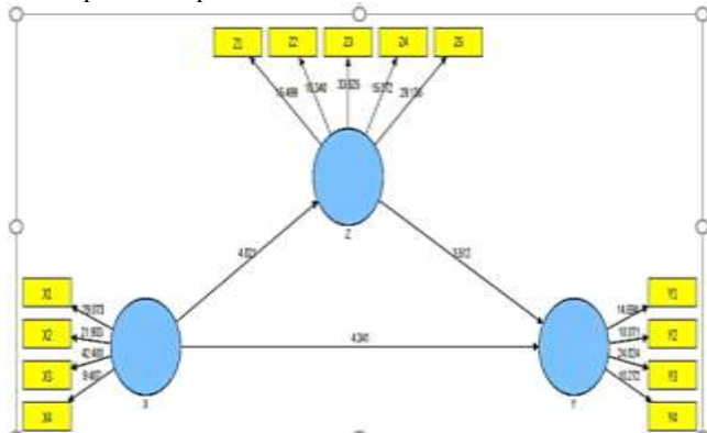
Gambar 4.2 Hasil analisis inner model
