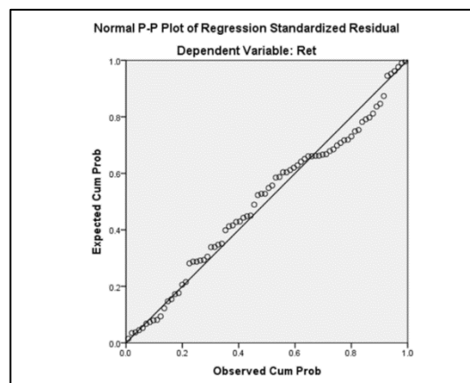
Figure 3. Normal Probability Plot (n=78)
