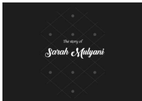
Gambar 3. Booklet CD
