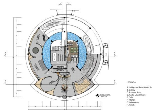
Gambar 6. Layout Perancangan Interior Museum Purbakala Patiayam, Kudus
