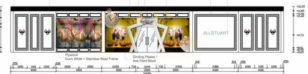
Gambar 27. Main Entrance lantai 2.
